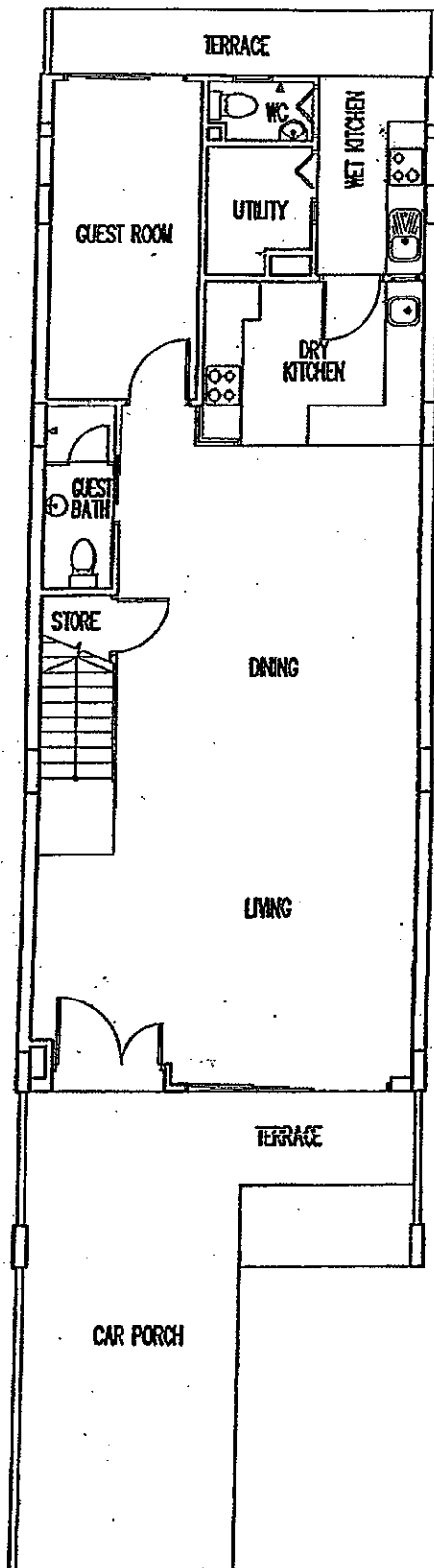
1ST STOREY PLAN
