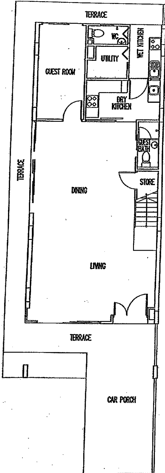
1ST STOREY PLAN
